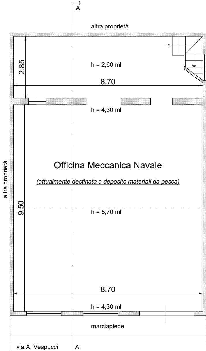
PIANO TERRA
